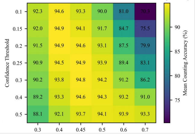
Fig. 4: Heatmap of mean counting accuracy across different confidence and Intersection over Union (IoU) threshold combinations.
